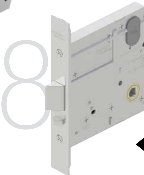
DKMS2902SSS PRIMARY MORTICE LOCK (MS2900 SERIES) 95 MM
