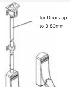
Exidor Panic Exit Device Accessory Extended Top Shoot Tube for Doors up to 3180mm EXIP0804SIL
