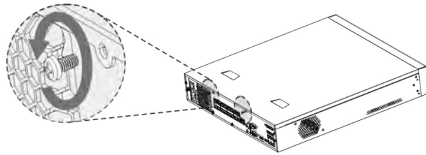
Figure 2-16 Remove screws
