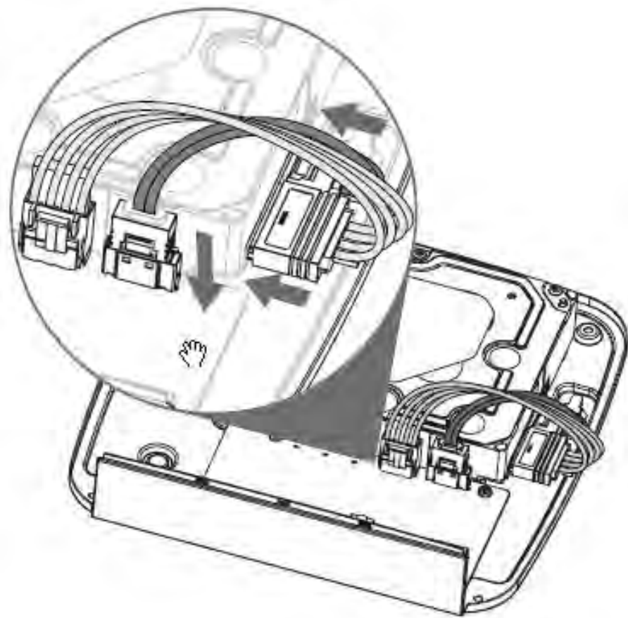
Figure 2-33 Connect cables
