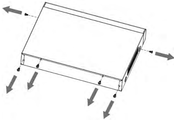
Figure 2-25 Remove cover
