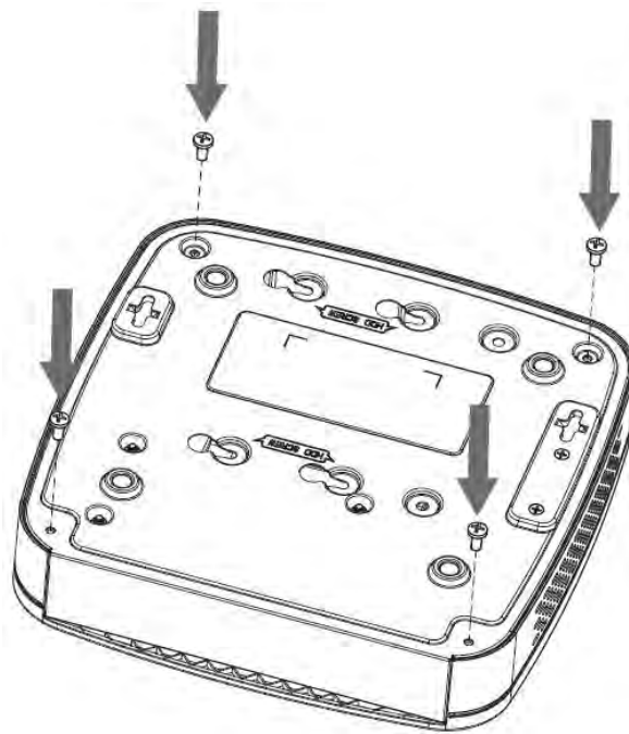
Figure 2-35 Fasten screws
