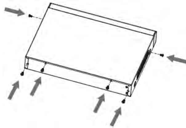
Figure 2-29 Fasten screws
