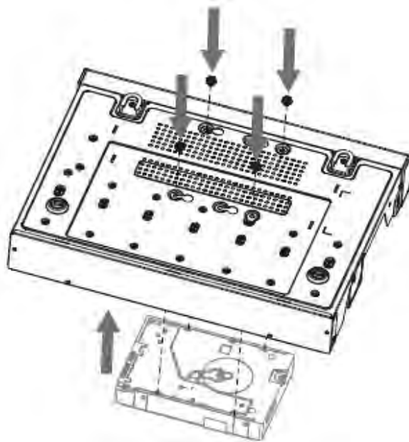
Figure 2-26 Fasten screws
