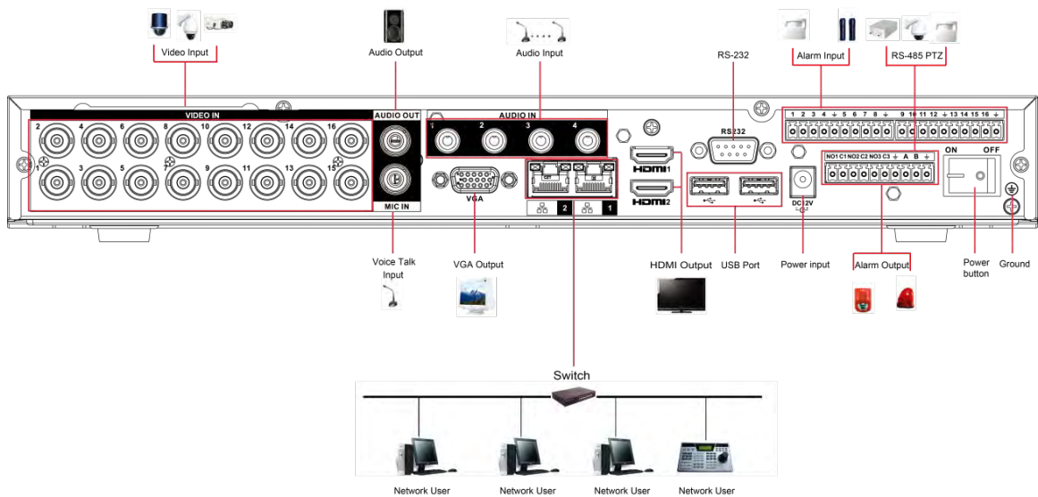
Figure 4-1 Connection diagram
