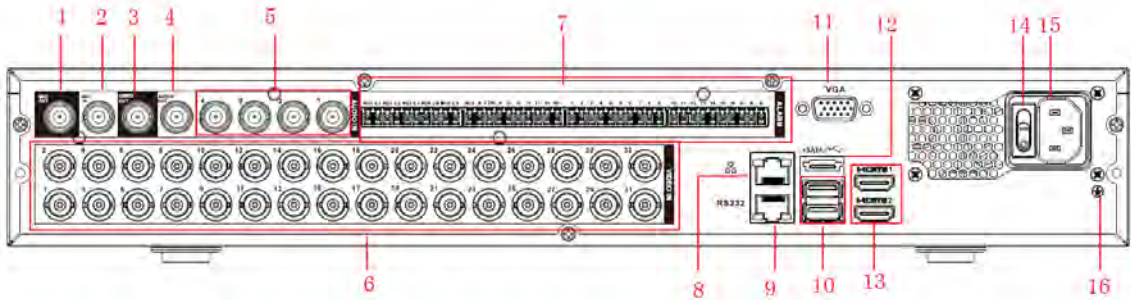
Figure 3-19 Rear panel (2)
