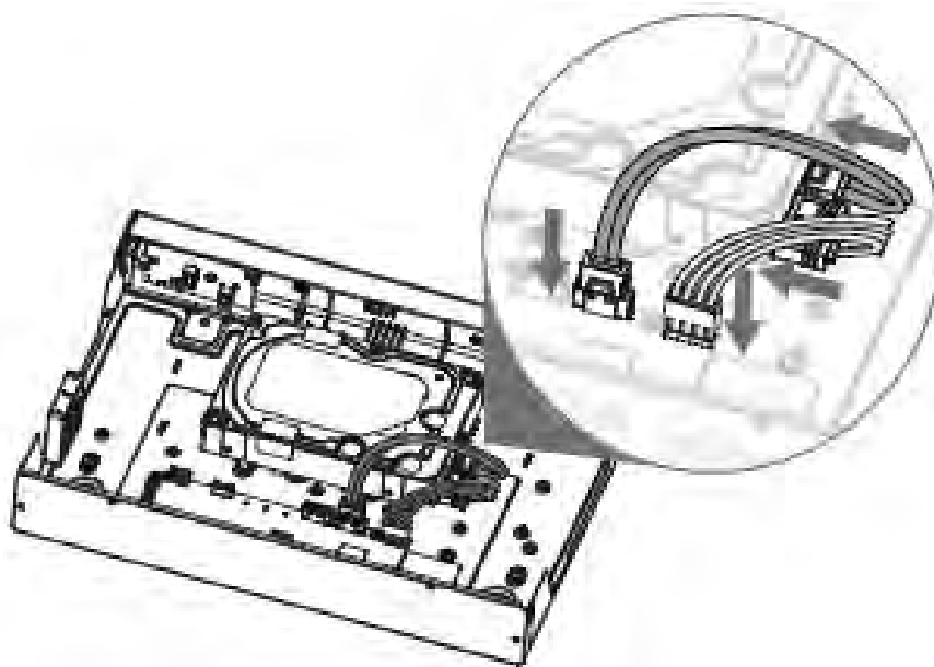
Figure 2-27 Connect cables
