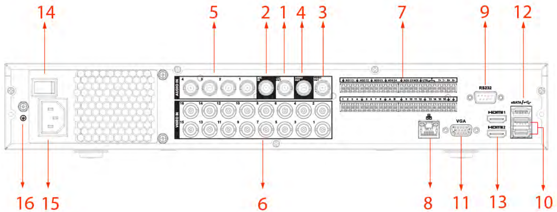
Figure 3-20 Rear panel (3)
