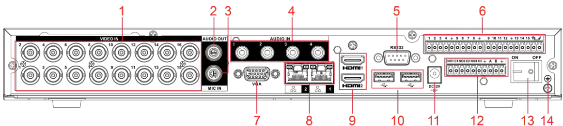
Figure 3-15 Rear panel
